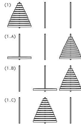
Figure 2.1: Recursively solving the towers of Hanoi problem.
